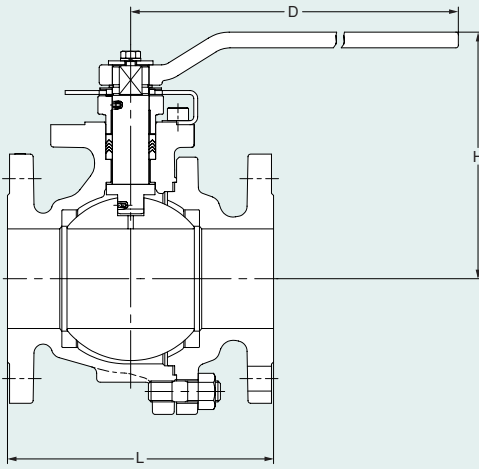
Dimensions of 150SCTDZ
